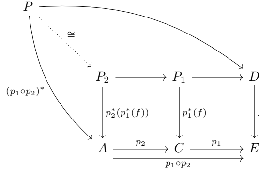
Figure 1: Pseudo functoriality of the pullback
