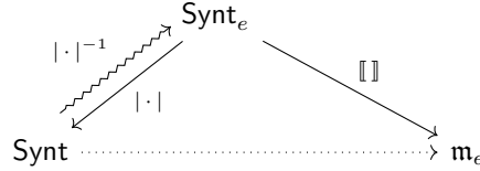
Figure 2: Relation of original and explicit theories and LCCC
